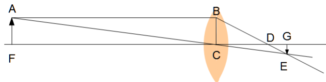
FIGURE 1. Formation of an image from a lens.
