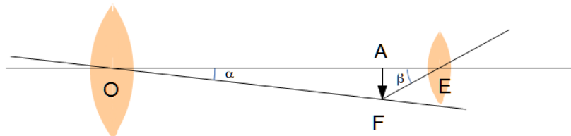
FIGURE 1. Optics of a refracting telescope.
