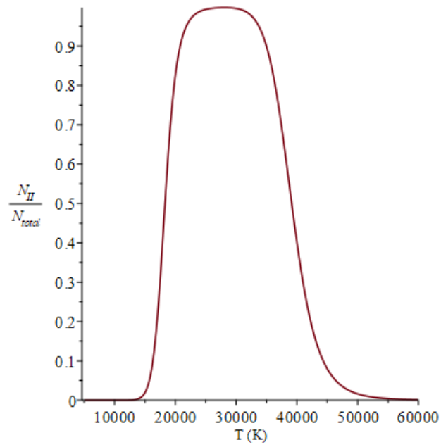
FIGURE 5. Fraction of singly ionized helium in a stellar interior.
