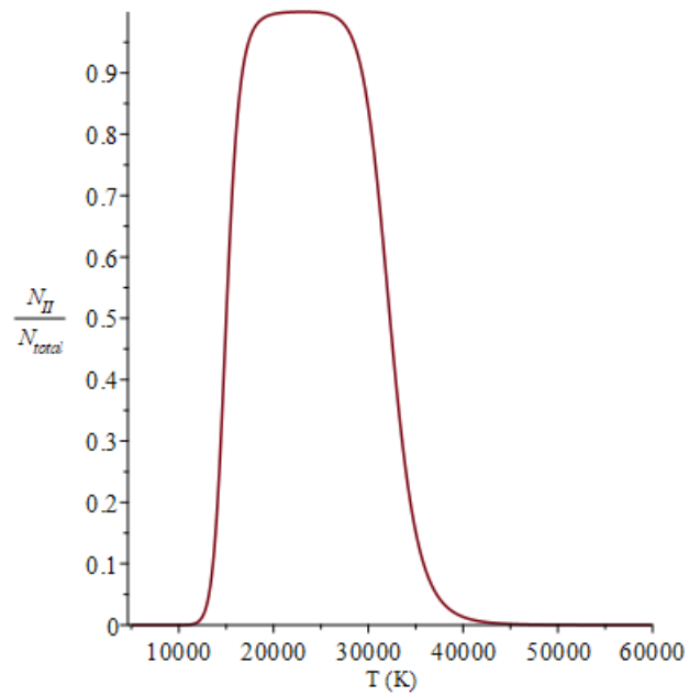
FIGURE 2. Fraction of singly ionized helium in a stellar atmosphere.
