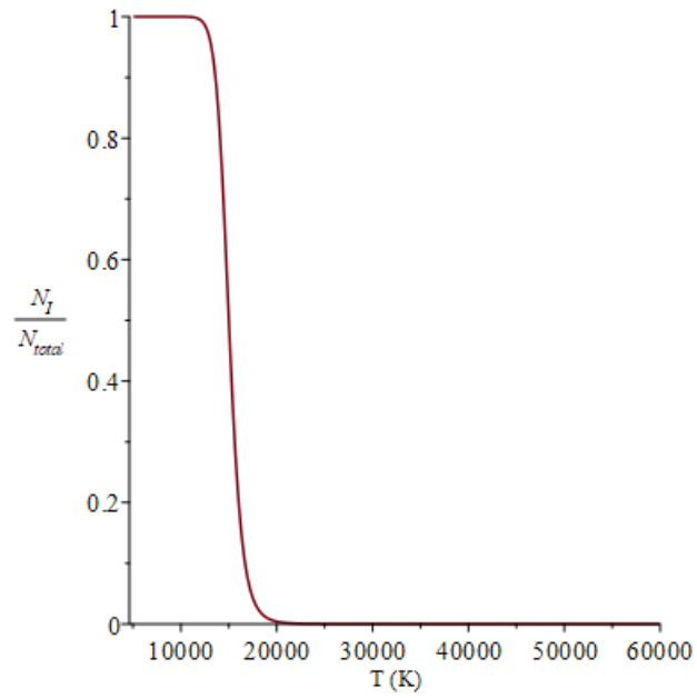
FIGURE 1. Fraction of neutral helium in a stellar atmosphere.
