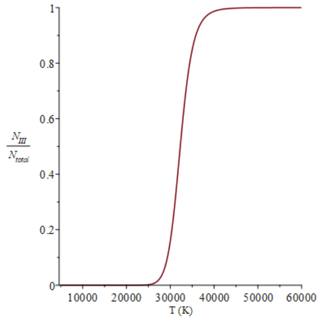
FIGURE 3. Fraction of doubly ionized helium in a stellar atmosphere.
