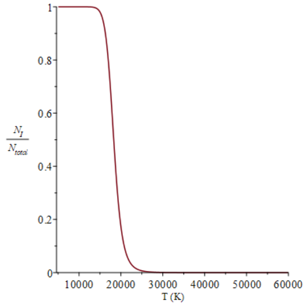
FIGURE 4. Fraction of neutral helium in a stellar interior.
