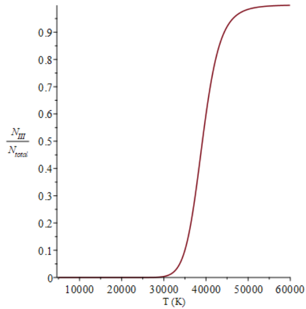
FIGURE 6. Fraction of doubly ionized helium in a stellar interior.
