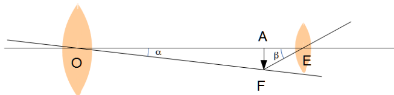
FIGURE 1. Magnification in a refracting telescope.
