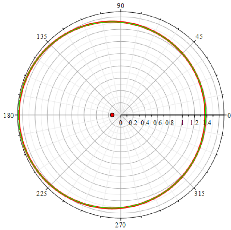
FIGURE 1. Circle (red) and ellipse (green) for Mars's orbit.
