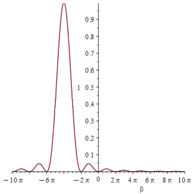
FIGURE 2. Diffraction from slit 2.
