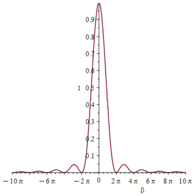
FIGURE 1. Diffraction from slit 1.
