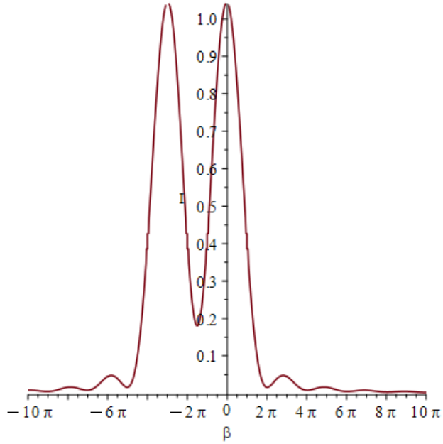
FIGURE 5. Slit 2 at \beta = -3\pi .
