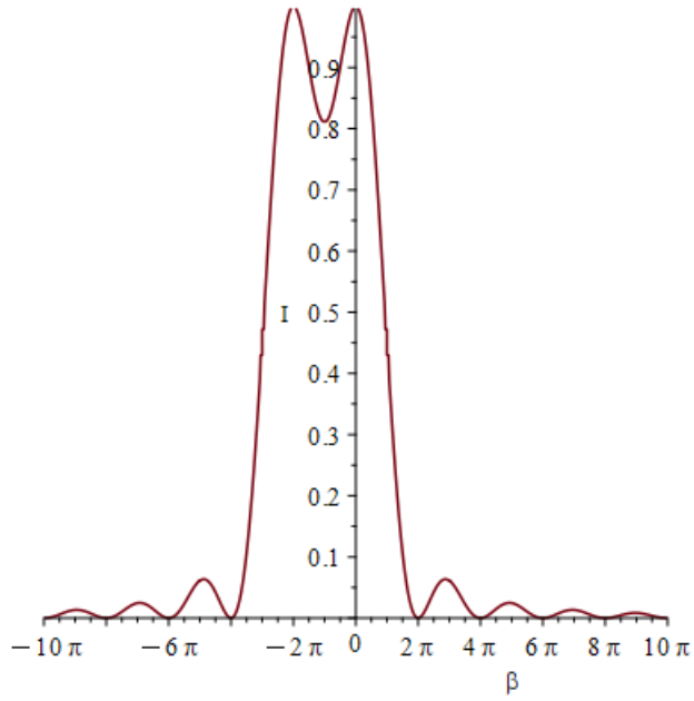
FIGURE 4. Slit 2 at \beta = -2\pi .
