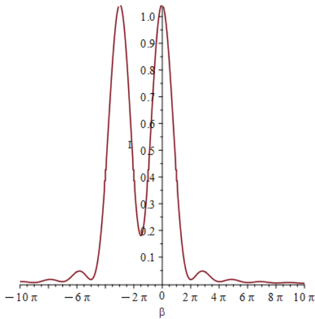
FIGURE 3. Slit 1 plus slit 2.
