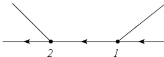
FIGURE 2. The diagram corresponding to :\overbrace{\psi_1^* \psi_1 \phi_1 \psi_2^* \psi_2 \phi_2}^{\quad}:
