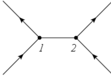
FIGURE 1. The diagram corresponding to :\psi_1^*\psi_1\overbrace{\phi_1\psi_2^*\psi_2\phi_2} :
