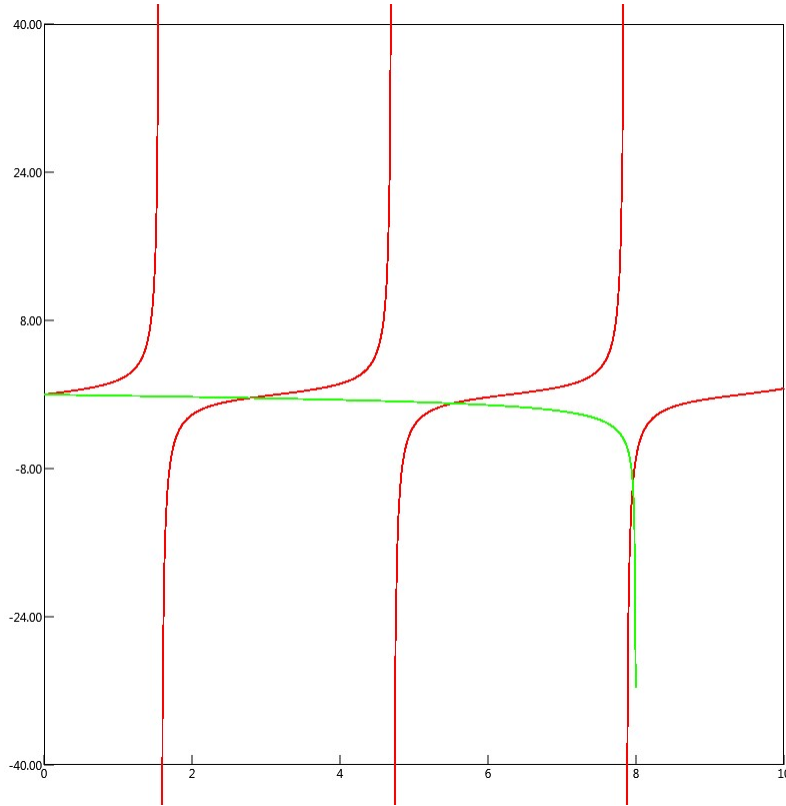
FIGURE 1. \tan z (red) and \frac{-1}{\sqrt{64/z^2-1}} .
