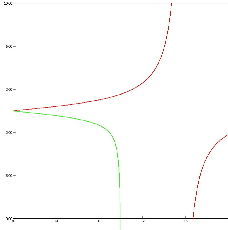
FIGURE 2. \tan z (red) and \frac{-1}{\sqrt{1/z^2-1}} .
