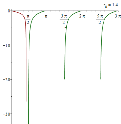
FIGURE 2. Plot of 20 for z_0 = 1.4 , with no intersections, so no bound states.
