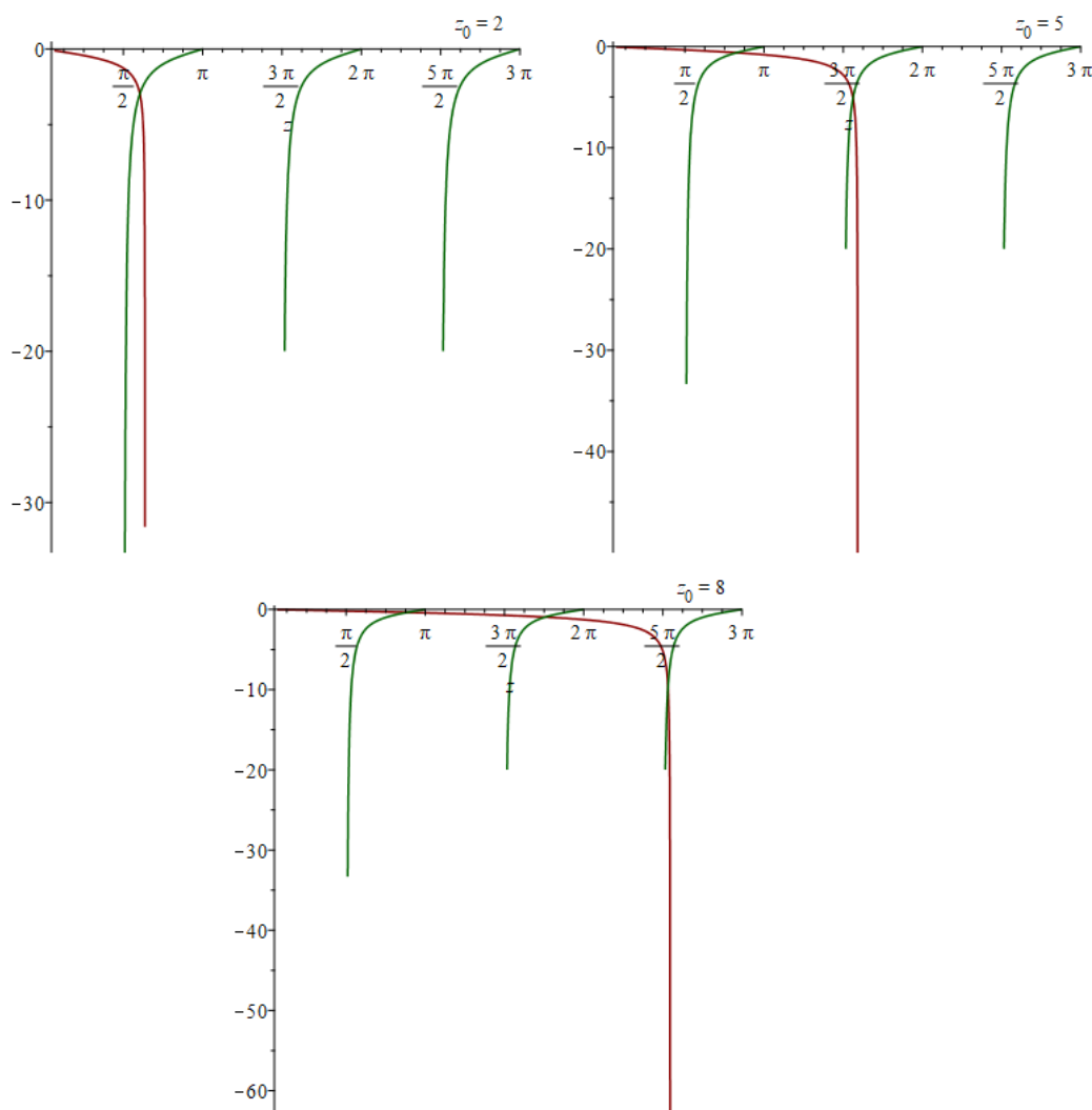
FIGURE 1. Plots of 20 for z_0 = 2, 5, 8 .
