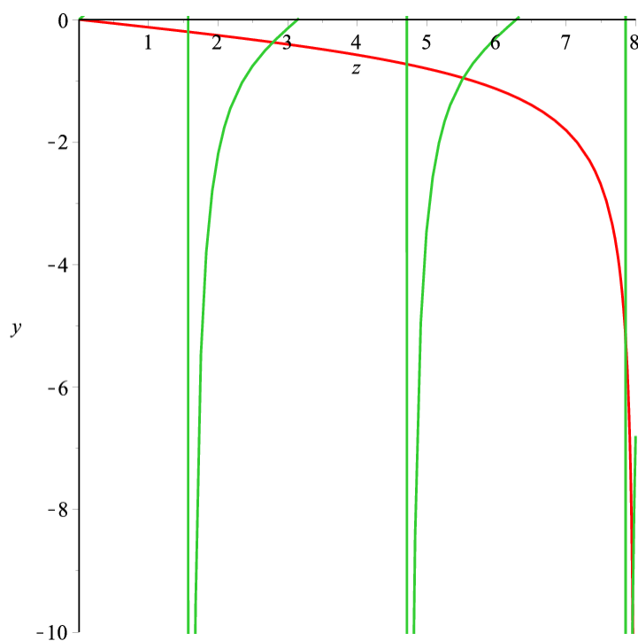
FIGURE 1. \tan(z) in green; -\frac{1}{\sqrt{64/z^2-1}} in red.
