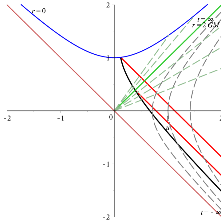
FIGURE 1. Kruskal-Szekeres spacetime diagram.
