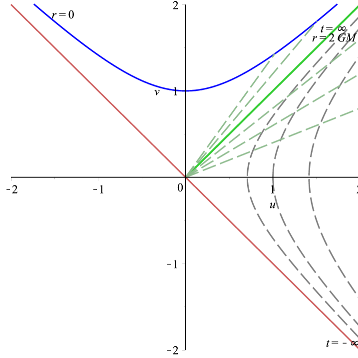
FIGURE 1. Kruskal-Szekeres diagram.
