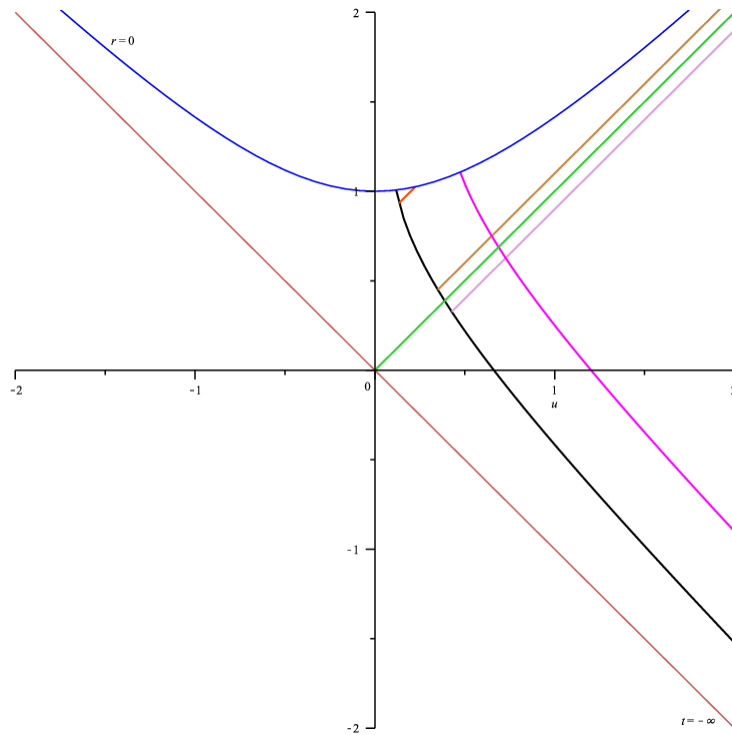
FIGURE 1. Kruskal-Szekeres diagram: spaceship falling into a black hole.
