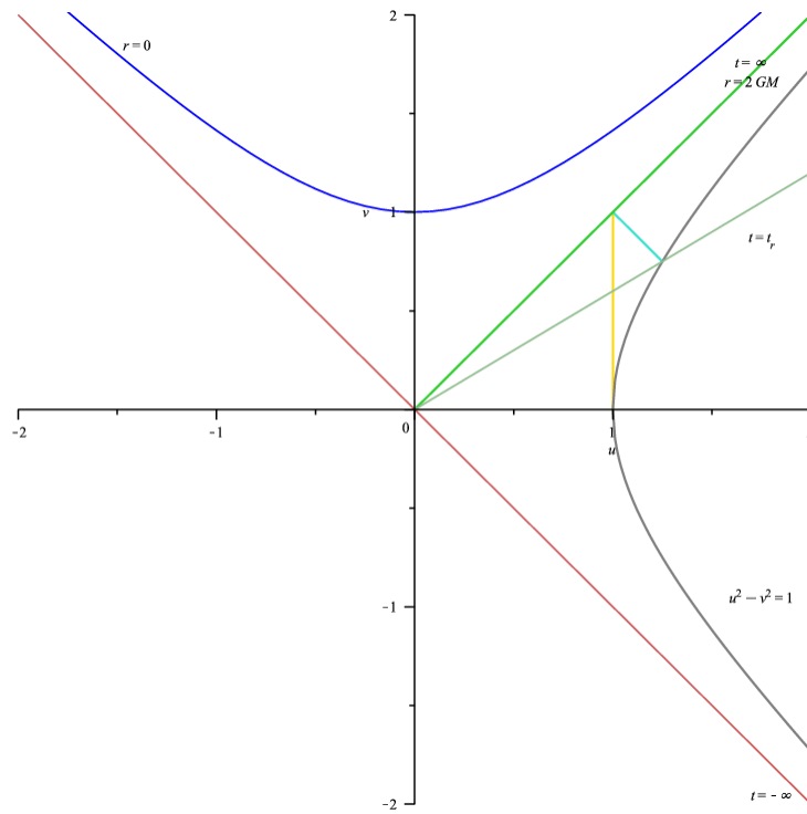
FIGURE 1. Kruskal-Szekeres diagram for a space shuttle being pulled into a black hole.
