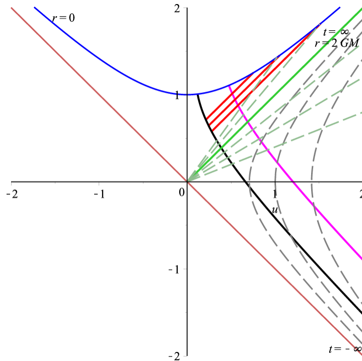
FIGURE 2. Kruskal-Szekeres diagram for a collapsing star.
