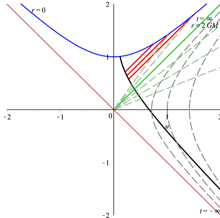
FIGURE 1. Kruskal-Szekeres diagram for photon torpedoes.
