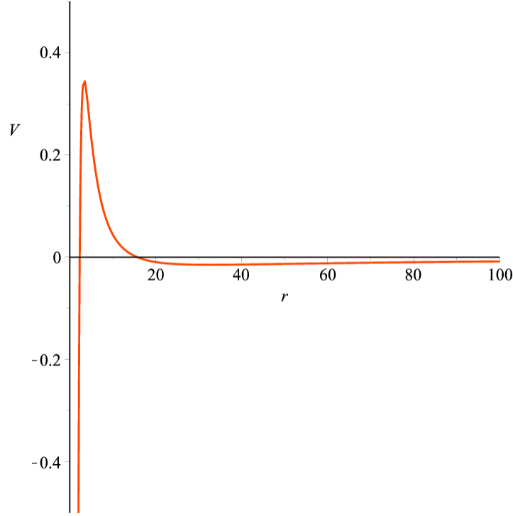
FIGURE 1. V from 19 versus r in GM units, with \ell = 6GM .
