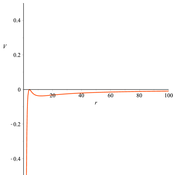
FIGURE 2. V from 19 versus r in GM units, with \ell = 4GM .
