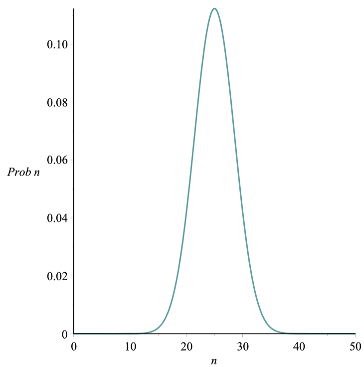
FIGURE 1. Probabilities of n heads in 50 coin flips.
