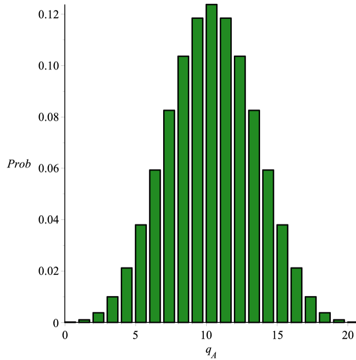
FIGURE 1. Probability distribution of q_A .
