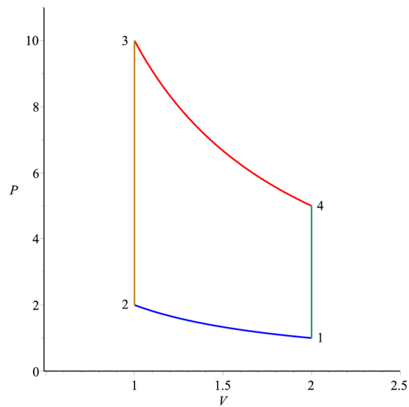
FIGURE 1. Stirling cycle.
