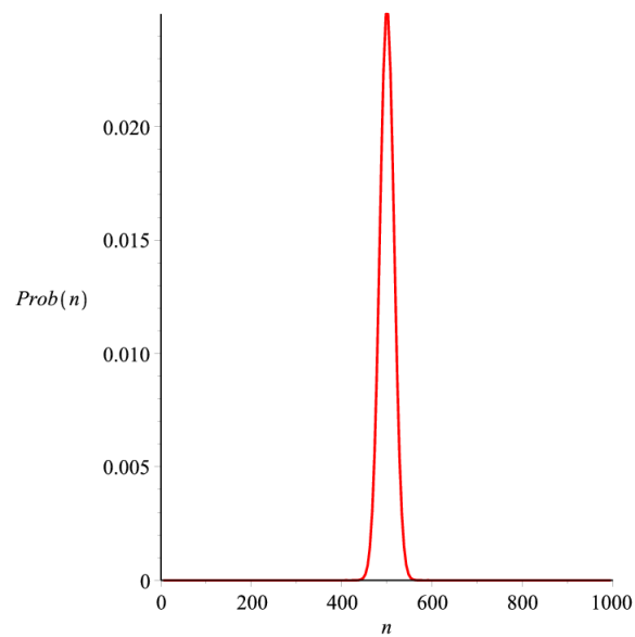
FIGURE 1. Probability of n heads in 1000 coin flips.
