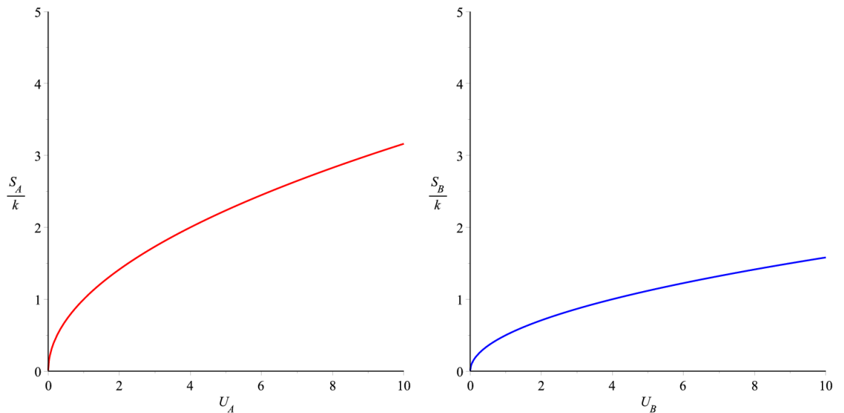
FIGURE 1. Systems A and B .
