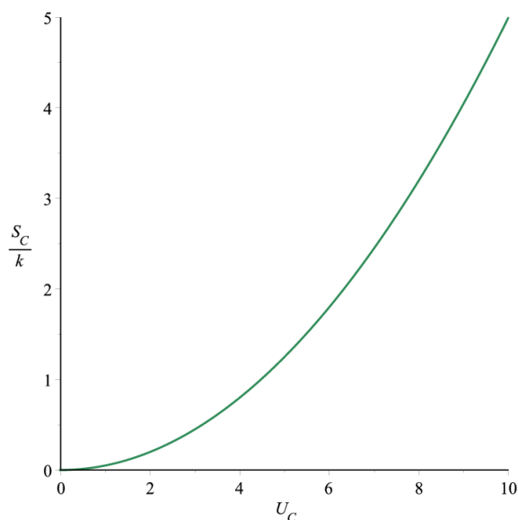
FIGURE 2. Negative heat capacity.
